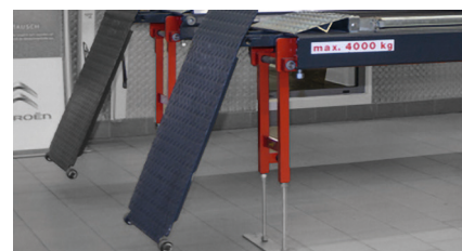
Supporting legs
